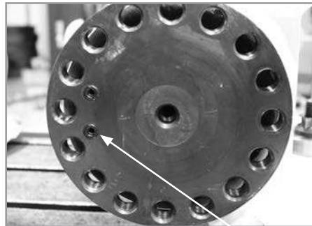
Port O-rings
